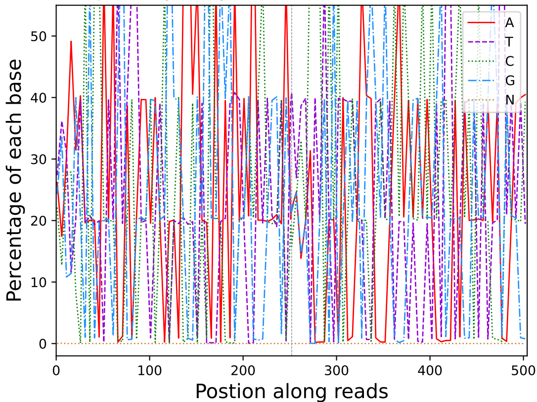
Base percentage along reads (R10725)
